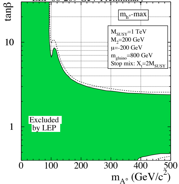
LEP 88-209 GeV Preliminary
