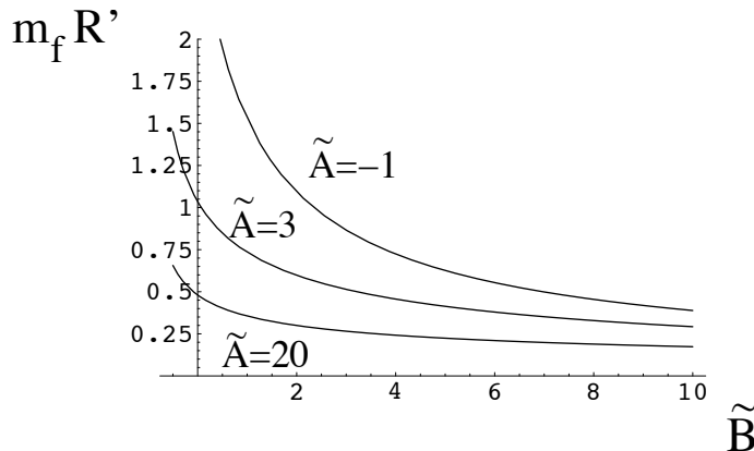
Figure 5: The mass of the IR localized fermion in units of the KK scale, 1/R' as a function of \tilde{B} for three values of \tilde{A} : -1 , 3 , 20 from top to bottom. We have chosen c = -1 and performed the integral in (7.12) from \tilde{z} = 0 to 1 .
