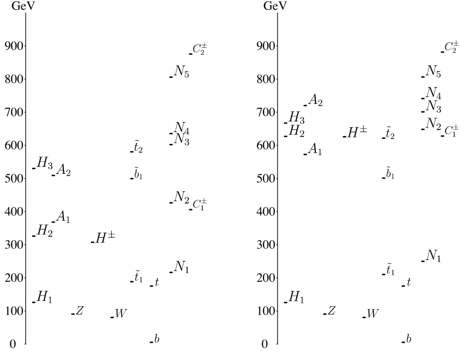
Figure 1: Light superpartners and Higgs particles for benchmark spectra 1 and 2 with a \tilde{t} NLSP.
